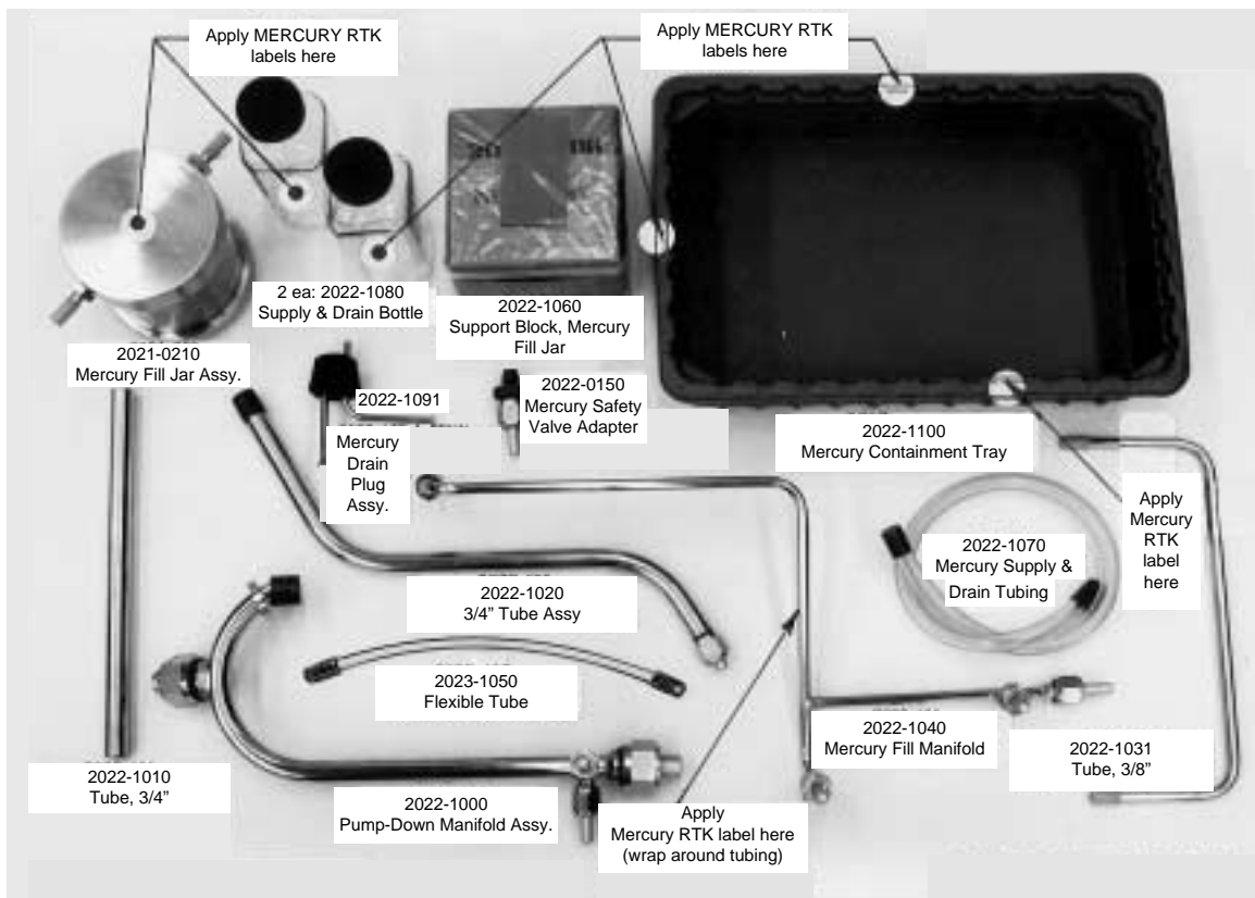
MERCURY FILL & PUMP-DOWN SYSTEM
